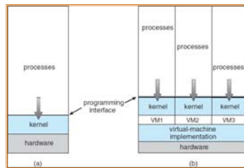
Non-virtual Machine Virtual Machine
